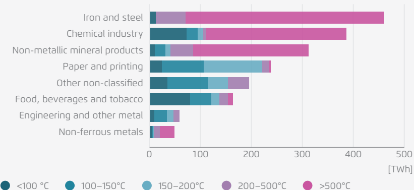
Estimated total final energy demand for process heating in 2019 by temperature and energy carrier in the EU-27 countries
